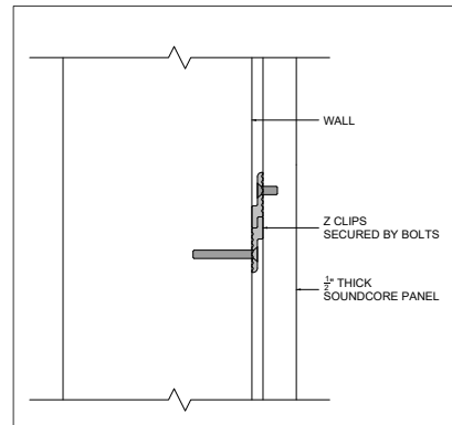
③ DETAIL VIEW
